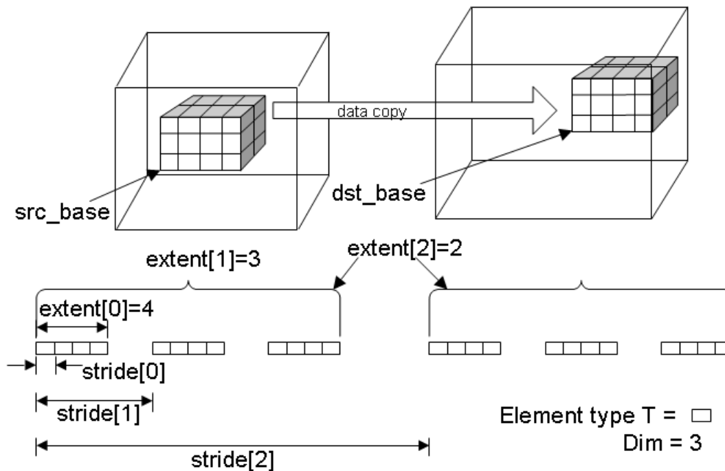
Figure 3: Example of strided one-sided communication.
