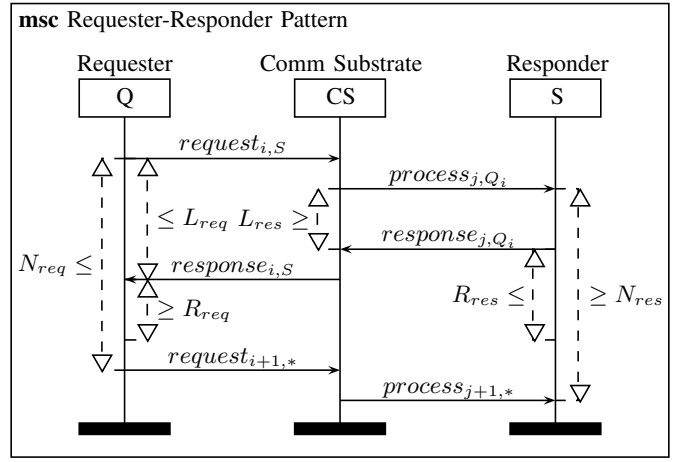
Fig. 2. Sequence of message flows and corresponding time periods (time progressing from top to bottom) in requester-responder pattern.
