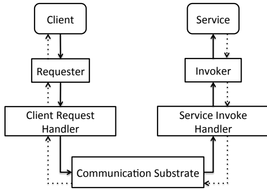
Fig. 3. Architecture of our implementation of communication patterns. Solid lines represent flow of data/request from client to service. Dotted lines represent the flow of data/response from the service to client.
