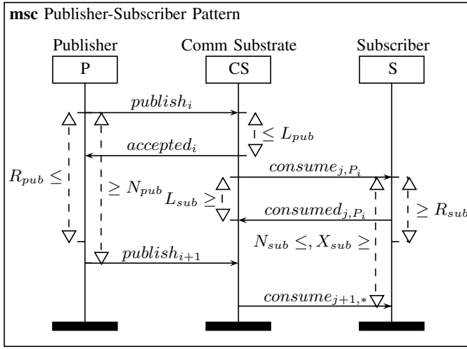
Fig. 1. Sequence of message flows and corresponding time periods (time progressing from top to bottom) in publisher-subscriber pattern.
